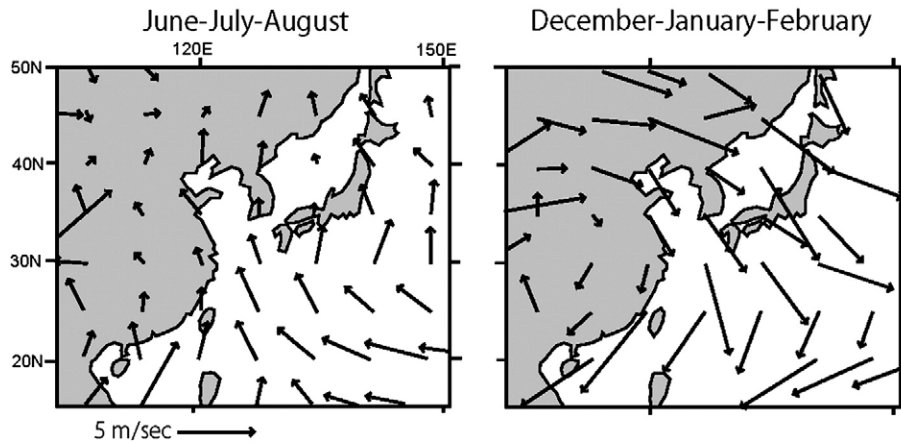
Fig. 1. Spatial distributions of observed mean surface wind (vectors) in East Asia for the periods June–August and December–February. Modified from Kitoh (2005).
