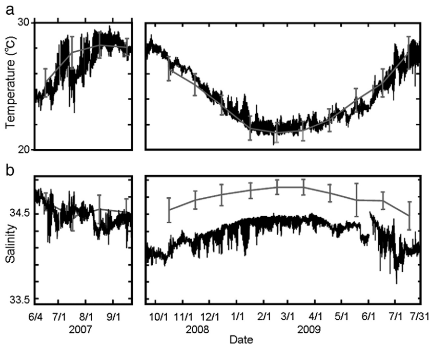
Fig. 4. (a) Observed temperatures within Shodokutsu cave. The observation period was from 3 June 2007 to 24 September 2007 and from 20 September 2008 to 31 July 2009. (b) Observed salinities within Shodokutsu cave. The observation period was from 3 June 2007 to 24 September 2007 and from 20 September 2008 to 31 July 2009. Seasonal variations in salinity (monthly mean values) at 30 m depth for the period 1906–2003 ( 1 \times 1 grid cells; 26\text{--}27^\circ\text{N} latitude and 127\text{--}128^\circ\text{E} longitude). Error bars represent one standard deviation ( 1\sigma ).
