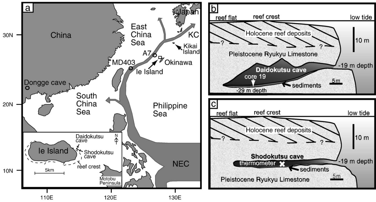
Fig. 2. (a) Location maps of Daidokutsu and Shodokutsu submarine caves at Ie Island, off Okinawa Japan, the locations of drill cores A7 (Sun et al., 2005; Xiang et al., 2007) and MD403 (Lin et al., 2006), and Dongge cave, China. NEC: North Equatorial Current; KC: Kuroshio Current. (b) Simplified cross-section of Daidokutsu cave, showing the location of core sample 19. (c) Simplified cross-section of Shodokutsu cave.
