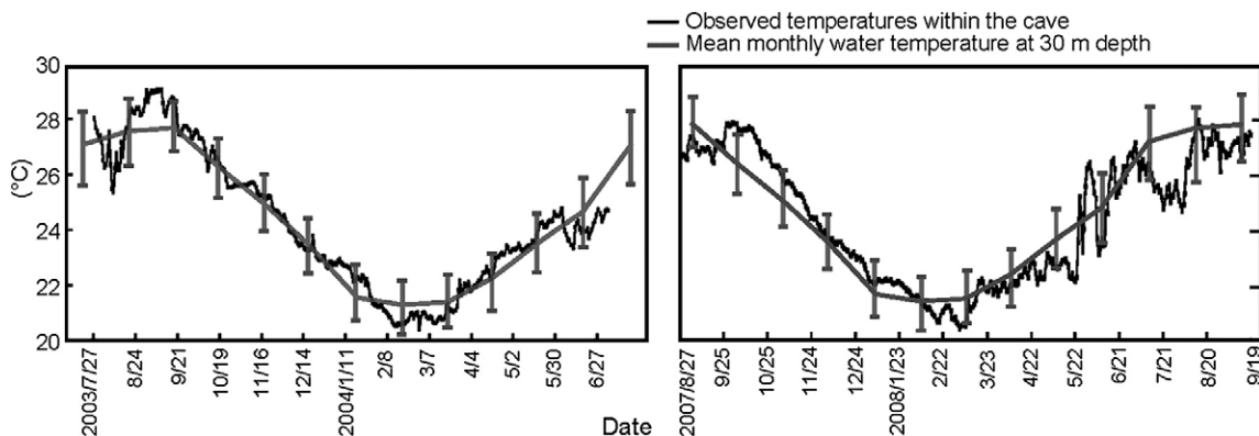
Fig. 3. Observed temperatures within Daidokutsu cave. The observation period was from 26 July 2003 to 6 July 2004, and from 27 August 2007 to 19 September 2008.
