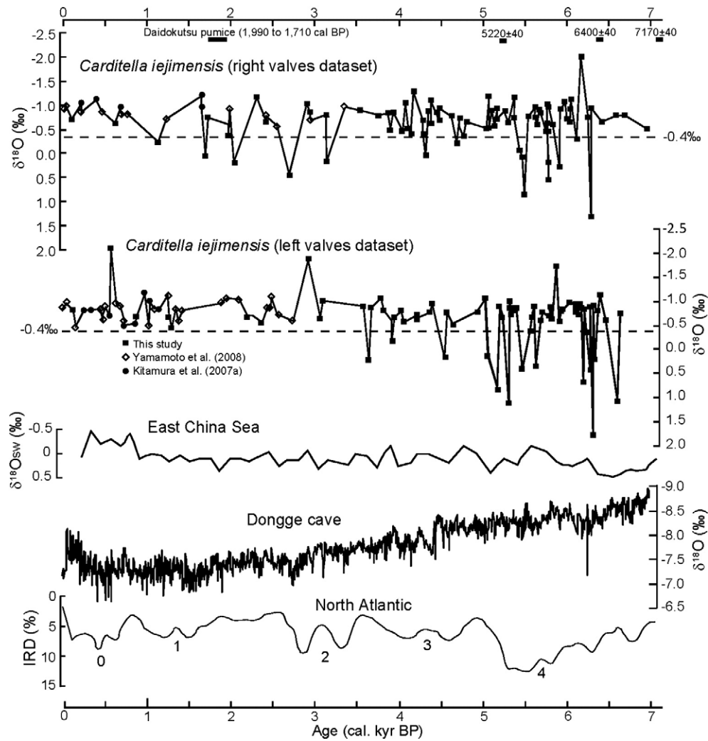
Fig. 7. Comparison of \delta^{18}\text{O} values of C. iejimensis from cored samples (present study) with the \delta^{18}\text{O}_{\text{seawater}} record from the East China Sea (Lin et al., 2006), stalagmite \delta^{18}\text{O} record from Dongge cave in southeast China (Wang et al., 2005), and record of ice-rafted debris from the North Atlantic (Bond et al., 2001). Note that the axes are inverted so that higher temperatures (lower \delta^{18}\text{O} ) are toward the top.
