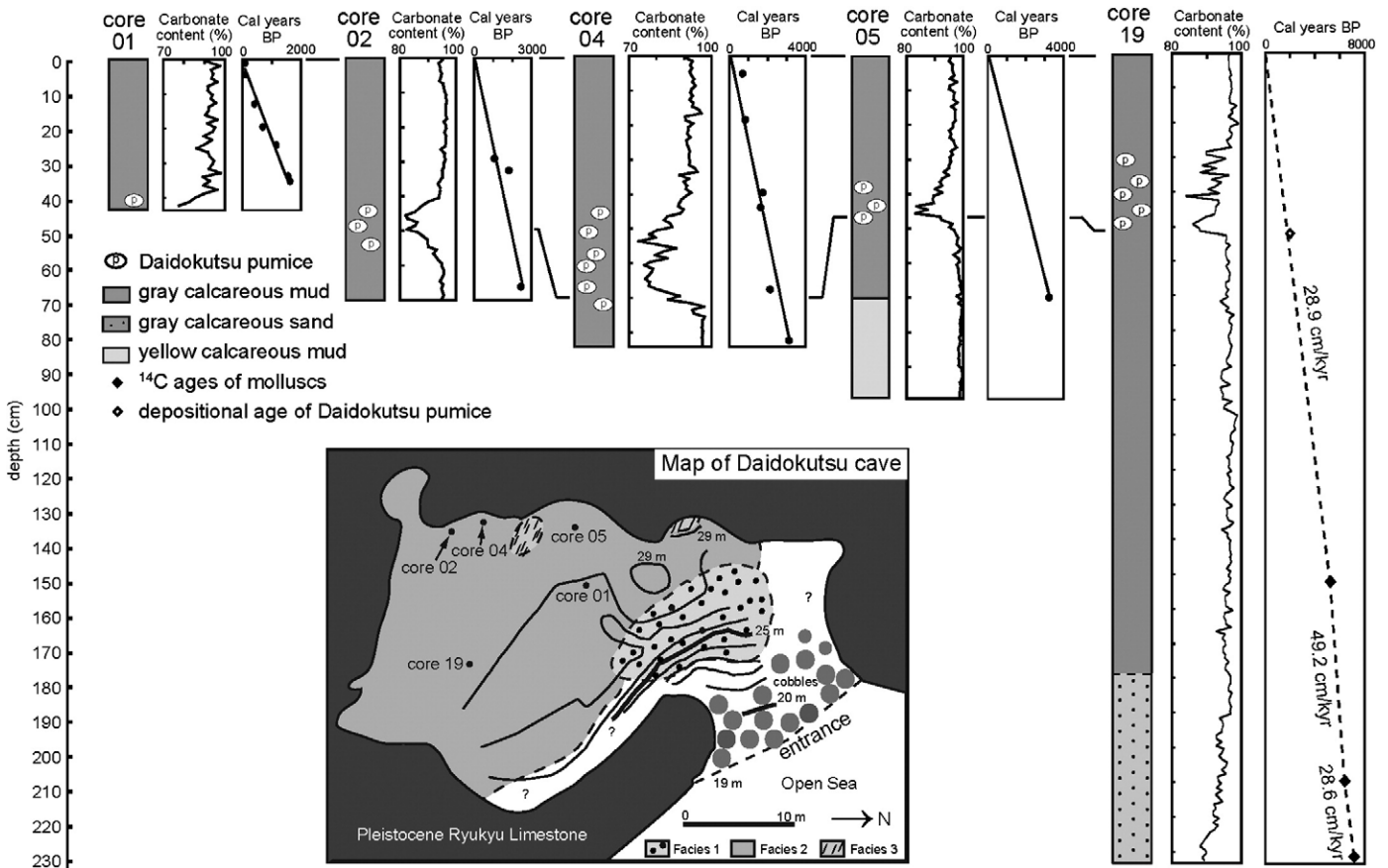
Fig. 6. Stratigraphic columns compiled for cores 01, 02, 04, 05, and 19 recovered from within Daidokutsu cave, showing the stratigraphic distribution of Daidokutsu pumice. Also shown is a map of the distribution of surface sediment facies within the cave. Facies 1, gray calcareous sand; Facies 2, gray calcareous mud; Facies 3, calcareous sand containing the skeletons of partly encrusted coralline sponges.
