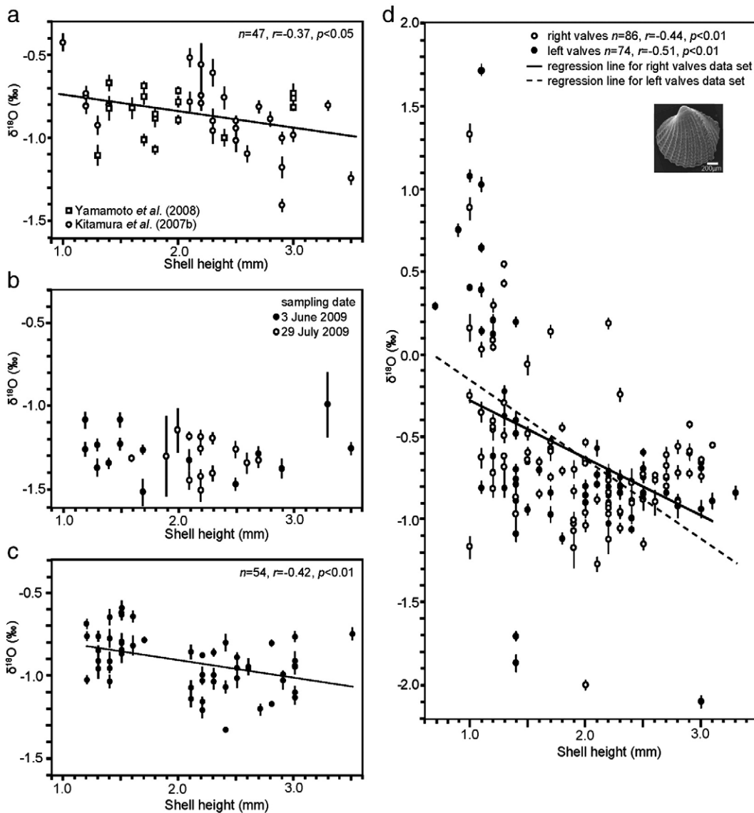
Fig. 5. Relationship between \delta^{18}\text{O} and the shell height of C. iejimensis . Error bars represent one standard deviation of a single \delta^{18}\text{O} analysis. Note that the vertical axes are inverted so that higher temperatures (lower \delta^{18}\text{O} ) are toward the top. (a) Empty shells from surface sediment within Daidokutsu cave; (b) living shells from surface sediment within Shodokutsu cave; (c) empty shells from surface sediment within Shodokutsu cave; (d) empty shells from core 19 within Daidokutsu cave.
